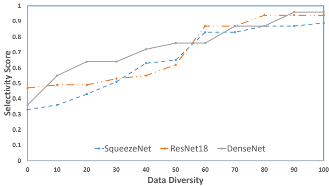
Fig. 2. Selectivity Score on Biased-Car dataset wrt data diversity
