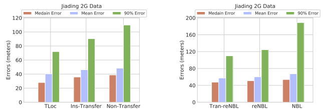
Fig. 11. Benefits of TLoc (from left to right). (a) Instance-based Transfer, (b) Fingerprinting-based localization.
