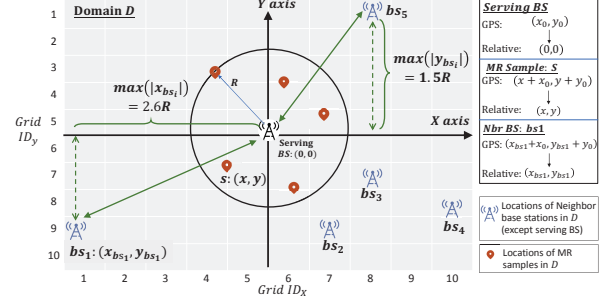
Fig. 2. Relative Coordinate Space
