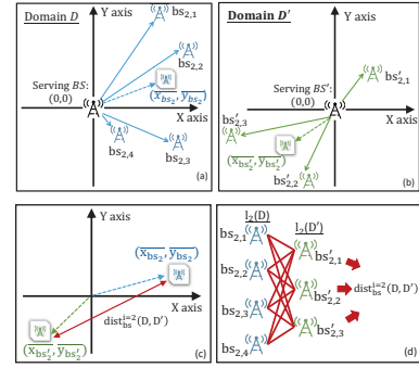
Fig. 5. Distance of BS Locations between Domains
