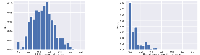
Fig. 6. Distribution of RSSI (left) and SignalLevel (right) Histogram Distance between Pairwise Domains.
