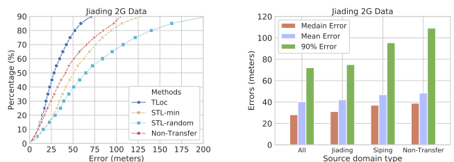
Fig. 12. Source Domain Selection (from left to right). (a) Four approaches, (b) Areas of source domains
