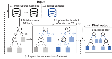
Fig. 9. Details of Structure Transfer in Random Forest.
