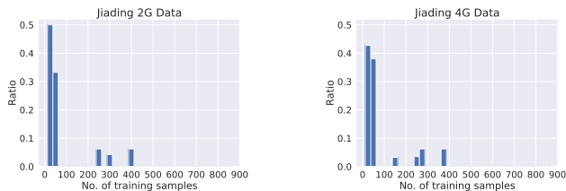
Fig. 10. Number of Training Samples in those Domains with Low-Accuracy.
