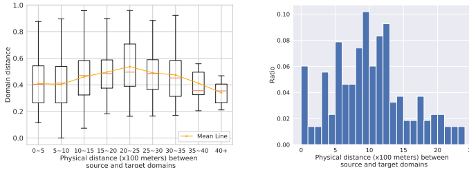
Fig. 8. Domain Selection (Jiading 2G). Left: Domain distance; Right: Top- k source domains
